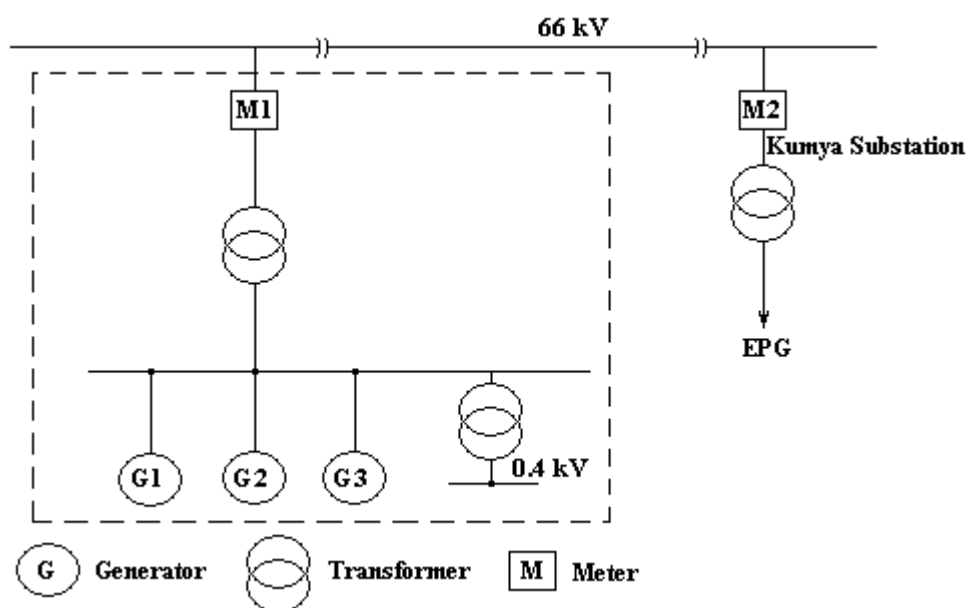
Fig.4. Monitoring system of Project
