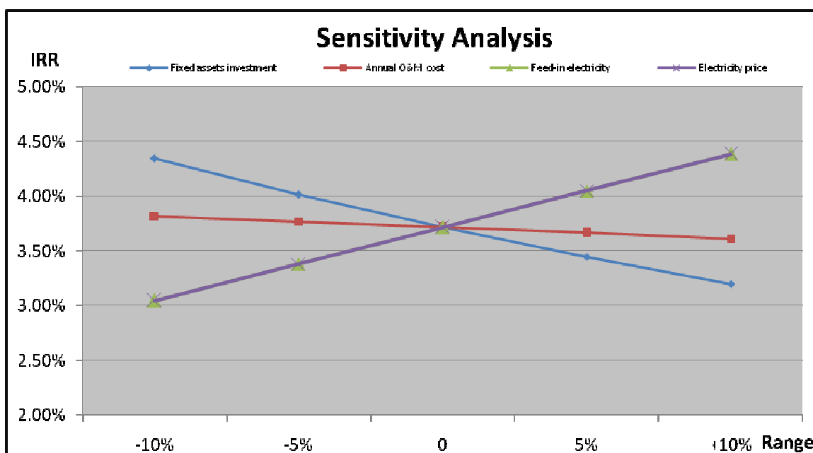
Fig.3 The IRR Sensitivity Analysis with the changes of Total Investment, Annual O&M Cost, Electricity price or Feed-in Electricity
